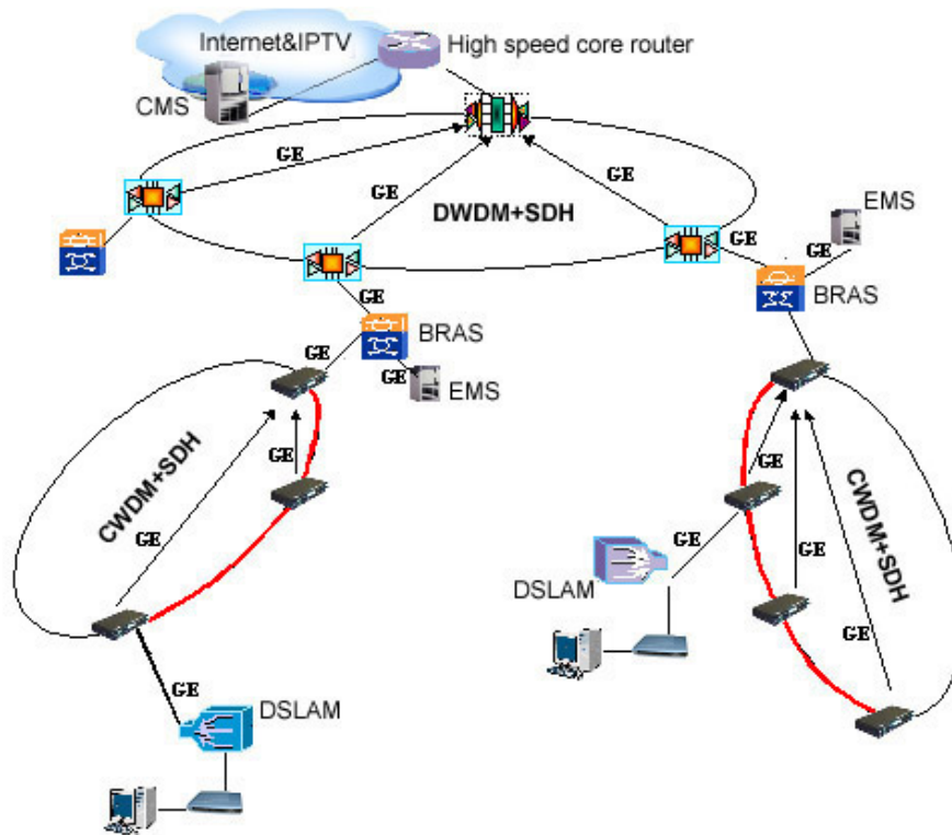
CWDM PLAN for Telecommunication industry
