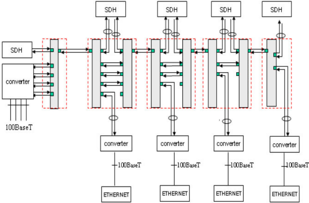
CWDM PLAN for Electric Power network
