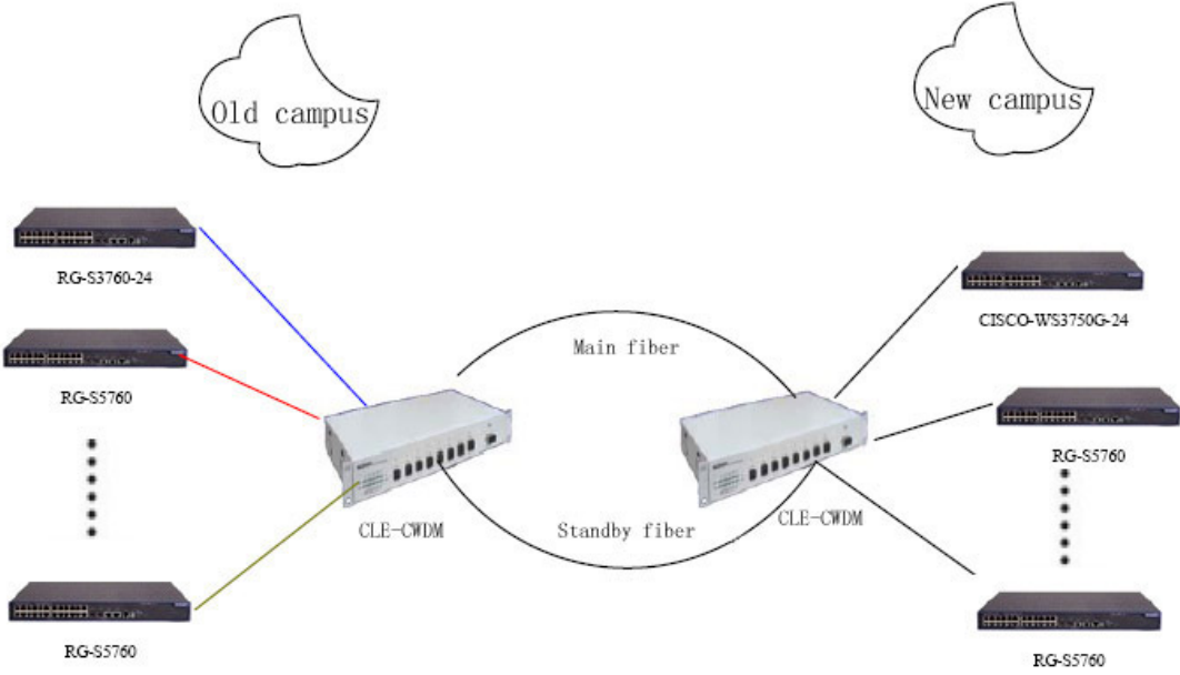
CWDM PLAN for campus network
